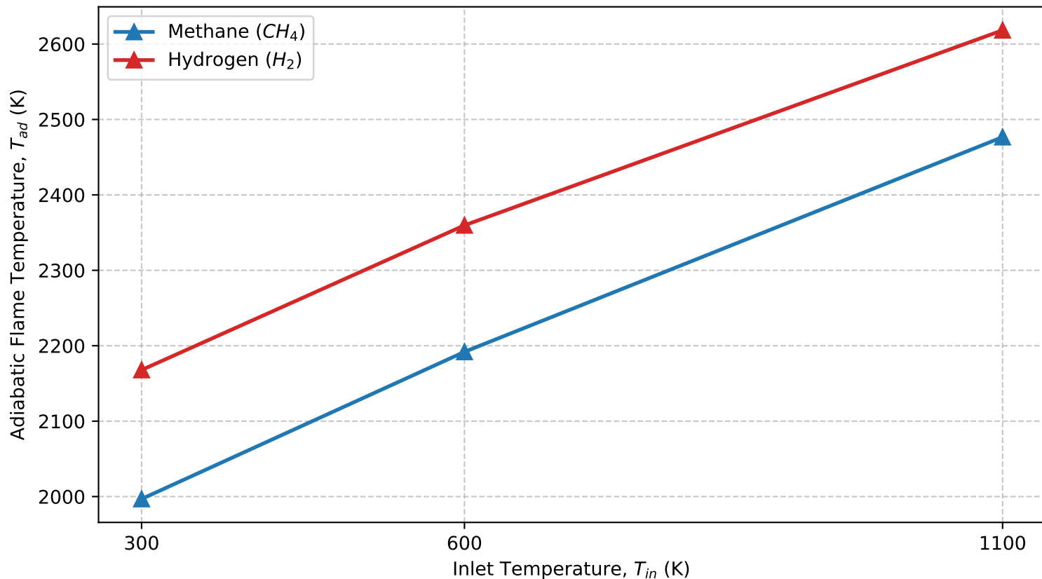
c) Adiabatic Flame Temp vs Inlet Temperature (Baseline: \phi=0.8 , P=1 bar)
